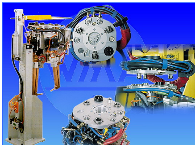
Left: Gun magazine with cover plate Middle above: robot side, below: Tool side Right: Side view with robot (above) and tool (below).
